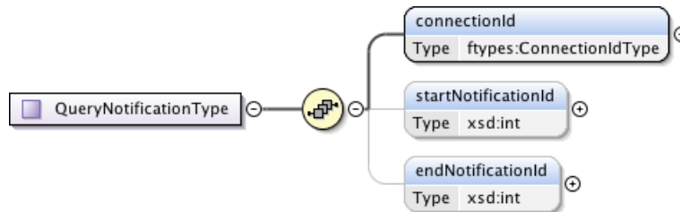
Figure 106 – QueryNotificationType .
