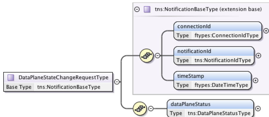
Figure 94 – DataPlaneStateChangeRequestType.
