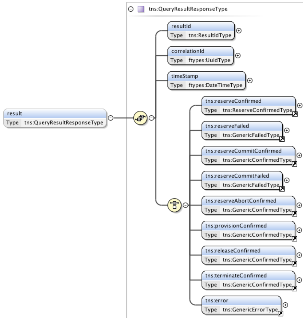
Figure 88 – QueryResultResponseType structure.
