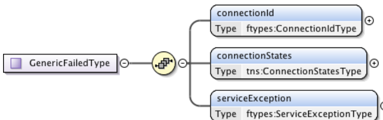
Figure 100 – GenericFailedType .
